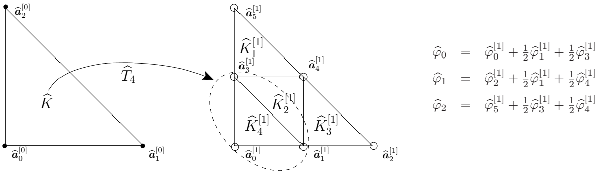
FIGURE 5. \mathbb{P}_1 -triangle refinement pattern and refinement equations.
