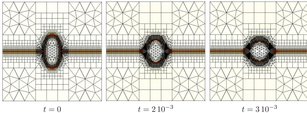
FIGURE 23. Tri/Quadr-angle- \mathbb{P}_1/\mathbb{Q}_1 . Time marching. h_{\text{interface}} = 0.4\epsilon
