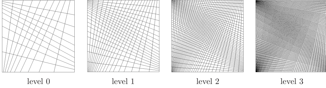
FIGURE 8. Quadrangle- \mathbb{Q}_1 . Nested meshes \mathcal{T}_j .
