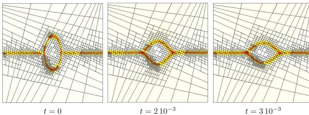
FIGURE 22. Quadrangle- Q_1 . Time marching. h_{\text{interface}} = 1.2\varepsilon
