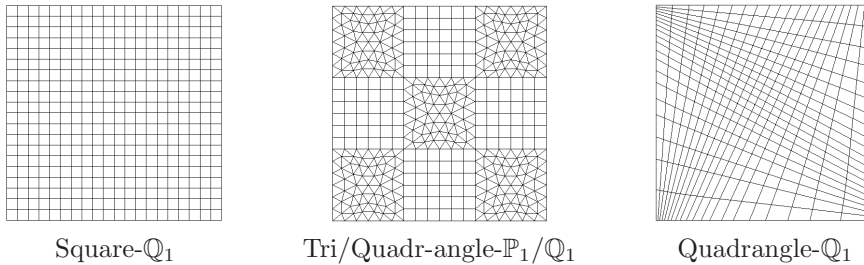
FIGURE 15. Initial meshes.
