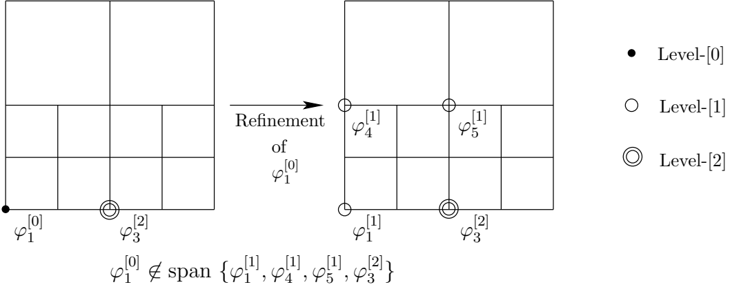
FIGURE 10. Refinement of multilevel basis is not lossless.
