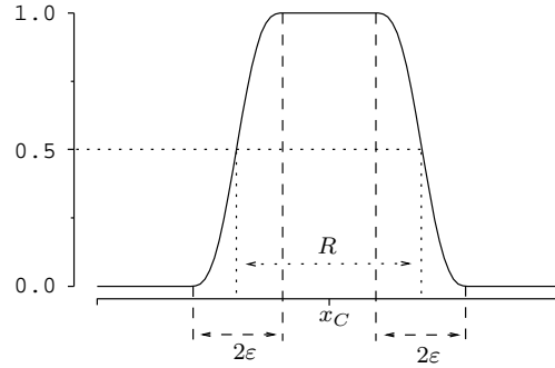
FIGURE 14. Exact solution of Problem 13, d = 1 .
