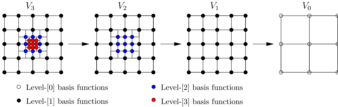
FIGURE 12. Example of coarsening : from V_3 to V_0 .
