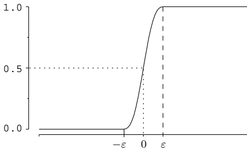
FIGURE 13. Function H_\varepsilon .
