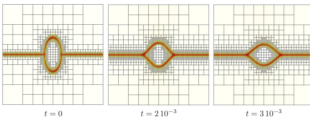
FIGURE 21. Square- Q_1 . Time marching. h_{\text{interface}} = \varepsilon
