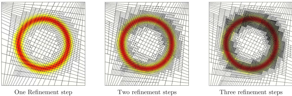
FIGURE 18. Quadrangle- Q_1 . Refined meshes.
