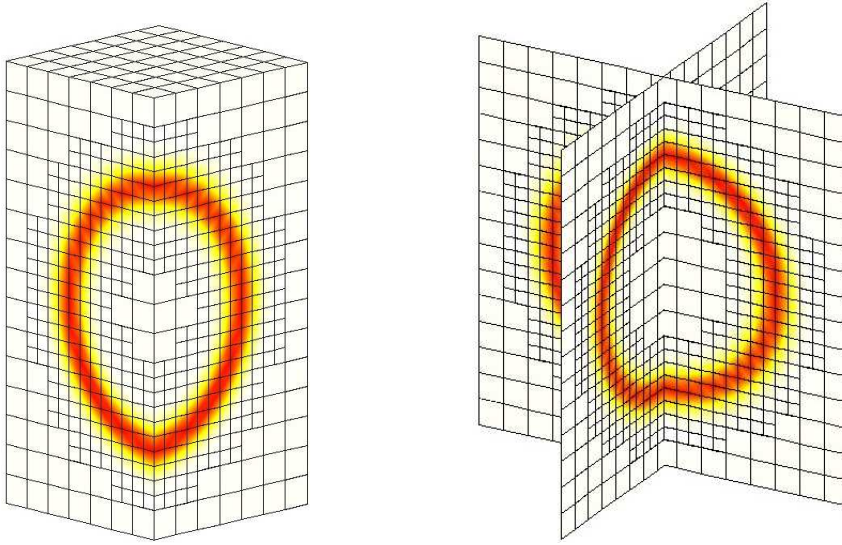
FIGURE 19. Refined mesh in 3D. One refinement step.
