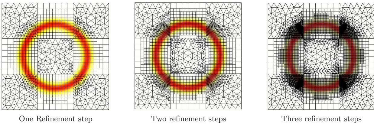
FIGURE 17. Tri/Quadr-angle- P_1/Q_1 . Refined meshes.
