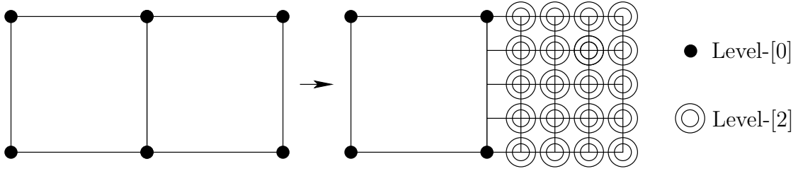
FIGURE 11. Refinement sequence forbidden by the One-level-difference rule.
