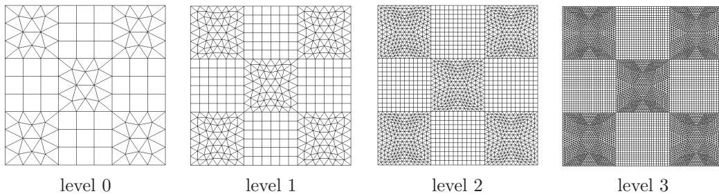
FIGURE 7. Tri/Quadr-angle- \mathbb{P}_1/\mathbb{Q}_1 . Nested meshes \mathcal{T}_j .
