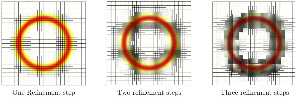
FIGURE 16. Square- Q_1 . Refined meshes.
