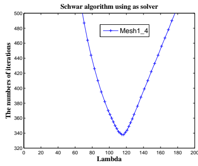
(a) Schwarz algorithm.
