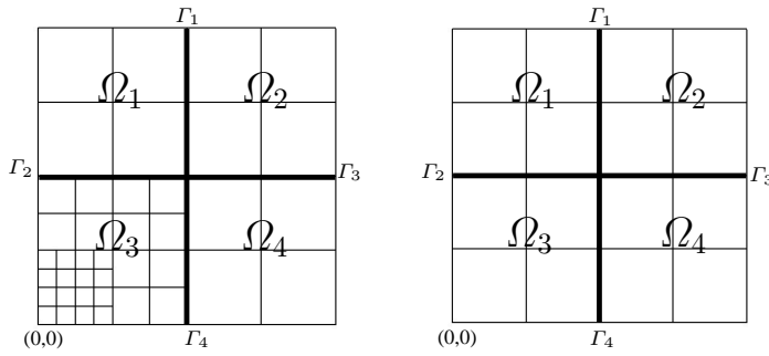
FIG. 5.2. The domain \Omega = [0, 1]^2 is divided in 4 subdomains. (Left) \text{Mesh}_1^3 . (Right) \text{Mesh}_1^4 .
