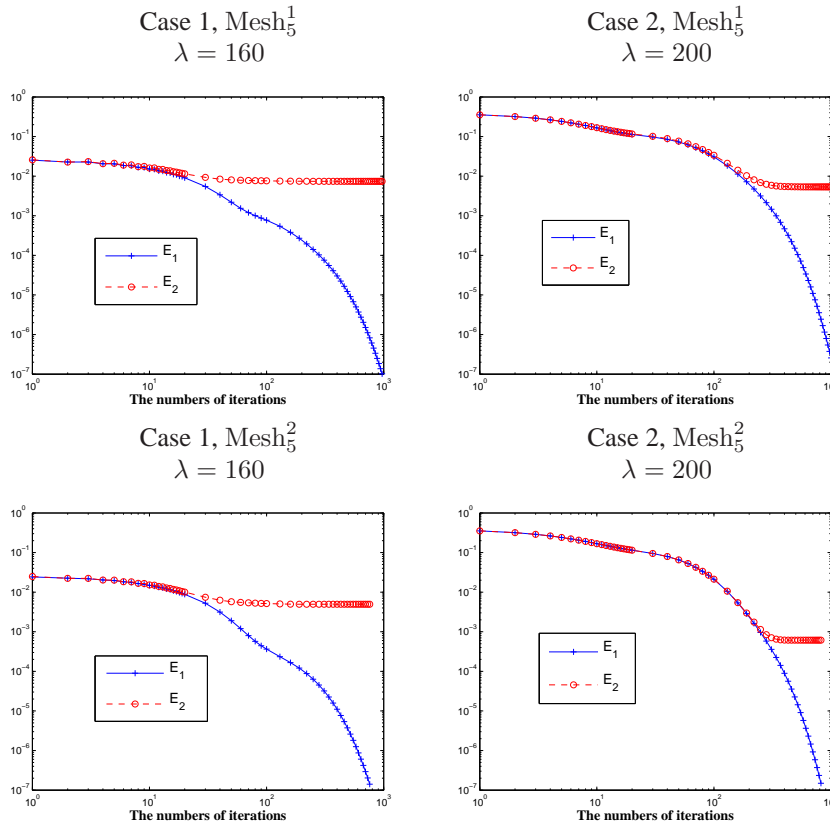
FIG. 5.6. Evolution of E_1 = \frac{\|u_n^{\mathcal{T}i} - u^{\mathcal{T}i}\|_2}{\|u^{\mathcal{T}i}\|_2} and E_2 = \frac{\|u_n^{\mathcal{T}i} - u_e\|_2}{\|u_e\|_2} as a function of the number of iterations. (Left) Case 1. (Right) Case 2.
