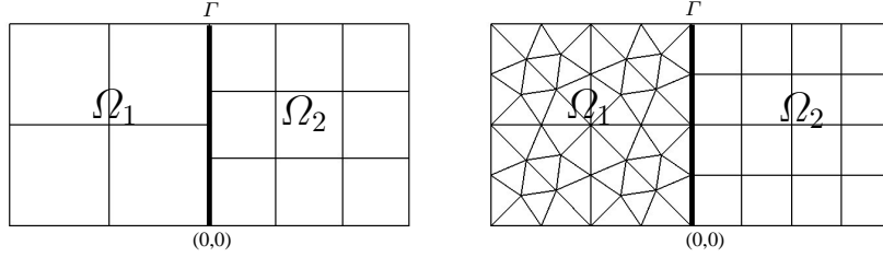
FIG. 5.1. The domain \Omega = [-1, 1] \times [0, 1] is divided in 2 subdomains. (Left) \text{Mesh}_1^1 . (Right) \text{Mesh}_2^1 .
