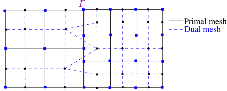
FIG. 4.6. The composite mesh \mathcal{T} corresponding to the 2 compatibles meshes of Figure 4.4.
