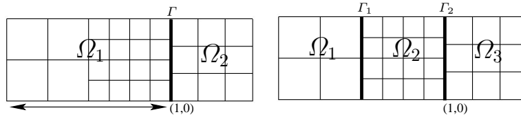
FIG. 5.4. The domain \Omega = [-1, 2] \times [0, 1] . (Left) \Omega is divided in 2 subdomains \text{Mesh}_1^6 . (Right) \Omega is divided in 3 subdomains \text{Mesh}_1^7 .
