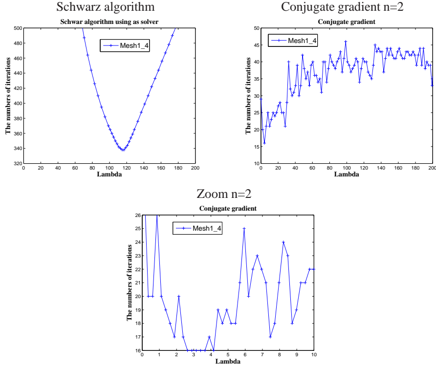
FIG. 5.12. The number of iterations to achieve an error of 10^{-8} as a function of \lambda . Case 7. (Left) For the Schwarz algorithm as a solver. (Middle and Right) For the conjugate gradient method with the Schwarz algorithm as a preconditioner.
