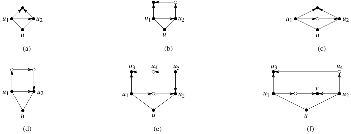
Figure 4: Configurations of Lemma 16
