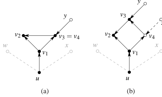
Figure 3: Configurations of Lemma 14
