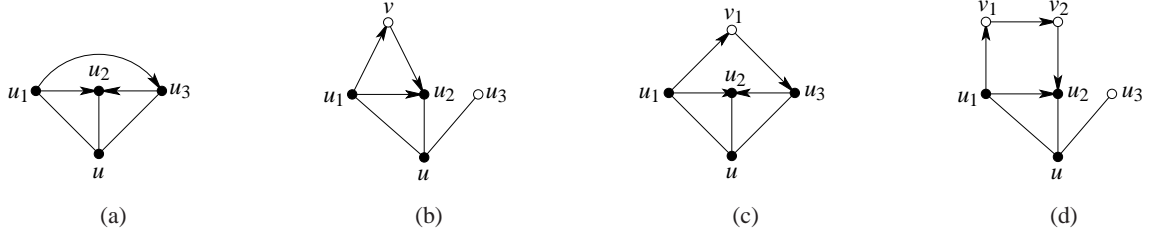
Figure 5: Configurations of Lemma 17
