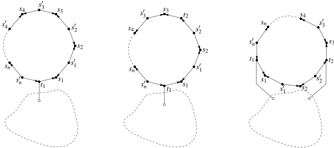
Figure 2: Graphs with a special cycle
