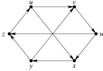
Figure 6: Cubic graph G with \chi'_o(G) = 6
