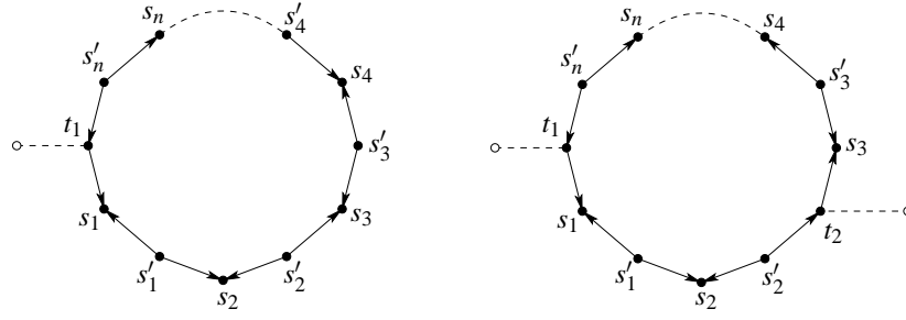
Figure 1: Two special cycles
