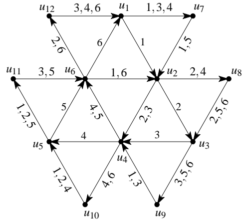
Figure 3: An oriented outerplanar graph with oriented chromatic index 7
