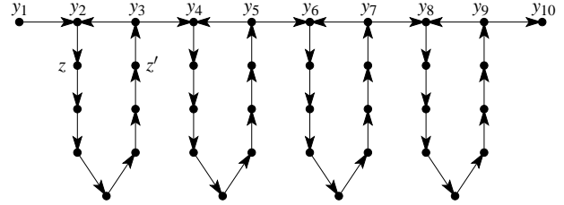
Figure 5: The configuration H for the proof of Theorem 3(3)
