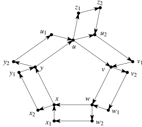
Figure 2: An oriented triangle-free outerplanar graph with oriented chromatic number 6
