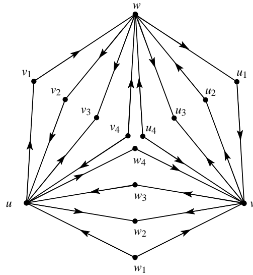
Figure 6: An oriented triangle-free partial 2-tree with oriented chromatic number 7
