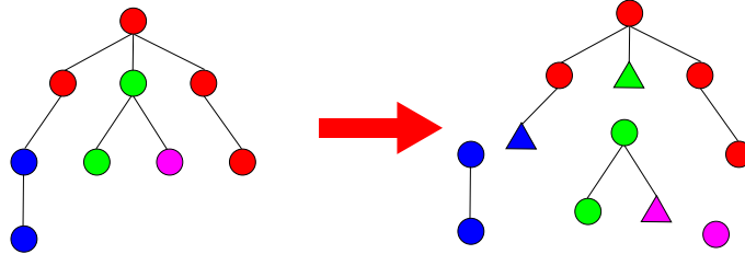
Fig. 7. Splitting the left tree into subtrees according to the colours of the nodes and addition of anchors (represented by triangles).
