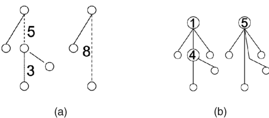
Fig. 7. (a) An example of edge fusion. (b) An example of node fusion.
