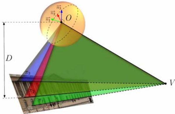
Figure 1. Geometry of the image and the vanishing plane, whose normal in O intersects the image on the vanishing point V
