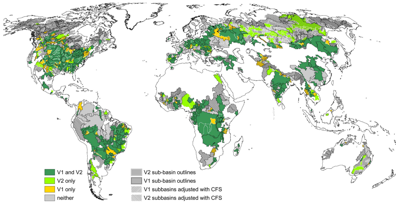
Fig. 3. Results of tuning WGHM 2.1 f variants V1 and V2. The color of the basins indicates whether each variant can compute observed long-term average river discharge at the stations by only adjusting the runoff coefficient. In the striped sub-basins, discharge needs to be adjusted by an additional station correction factor CFS.
