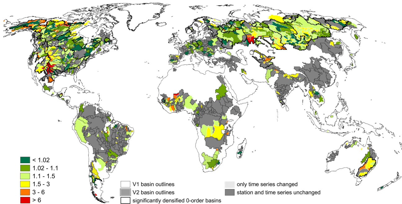
Fig. 5. Value of additional discharge information for simulating long-term average discharge (renewable water resources). The corrected basin-specific SDF of WGHM 2.1f variant V1 quantifies the increase in V2 model performance, i.e. the error in V1 that can be resolved by applying V2. SDF is only depicted at locations where V2 comprises supplemental information (additional stations or prolonged time series) as compared to V1; all other sub-basins are shown in grey. SDF values close to one indicate that performance gains by applying V2 are low. High SDF values indicate high value of additional discharge information.
