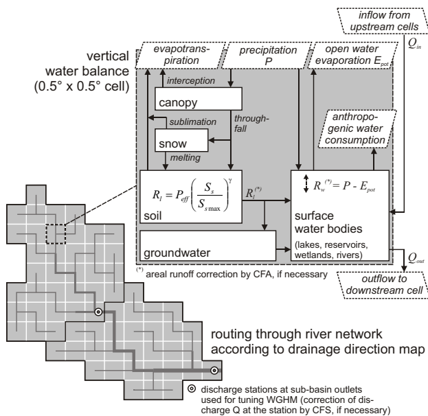
Fig. 2. Schematic representation of the global hydrological model WGHM. In the vertical water balance, runoff from land areas ( R_l ) is calculated as a function of effective precipitation ( P_{eff} : snowmelt + throughfall), soil saturation (actual storage S_s / maximum storage S_{s,max} ) and the tuning parameter \gamma . R_l and runoff from surface water bodies ( R_w ) are first routed through storages within the cell (groundwater, lakes, reservoirs, wetlands and rivers) and then transferred to the downstream cell, according to the drainage direction map. The parameter \gamma is adjusted in order to fit long-term average simulated discharge to observed discharge. In case \gamma does not suffice to adjust discharge, two correction factors are inserted successively: areal correction factor (CFA) to adjust runoff in the vertical water balance ( R_l , R_w ) and station correction factor (CFS) to fit river discharge ( Q ) at the outlet of a sub-basin.
