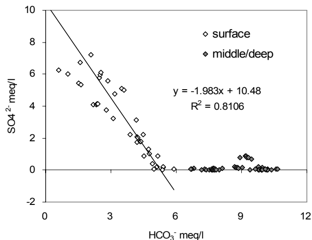
Fig. 9. Relationship between SO_4^{2-} vs. HCO_3^- concentration from groundwater samples collected at reed sub-unit. The equation and the coefficient of determination refers to the linear regression found for the surface samples.
