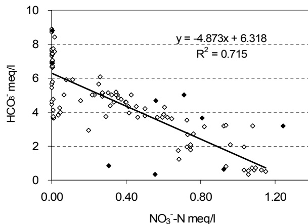
Fig. 8. Linear regression between NO_3^- -N and HCO_3^- concentration in poplar sub-unit groundwater samples. Solid dots represent an intense rainy event (December 2003) not included in the regression.
