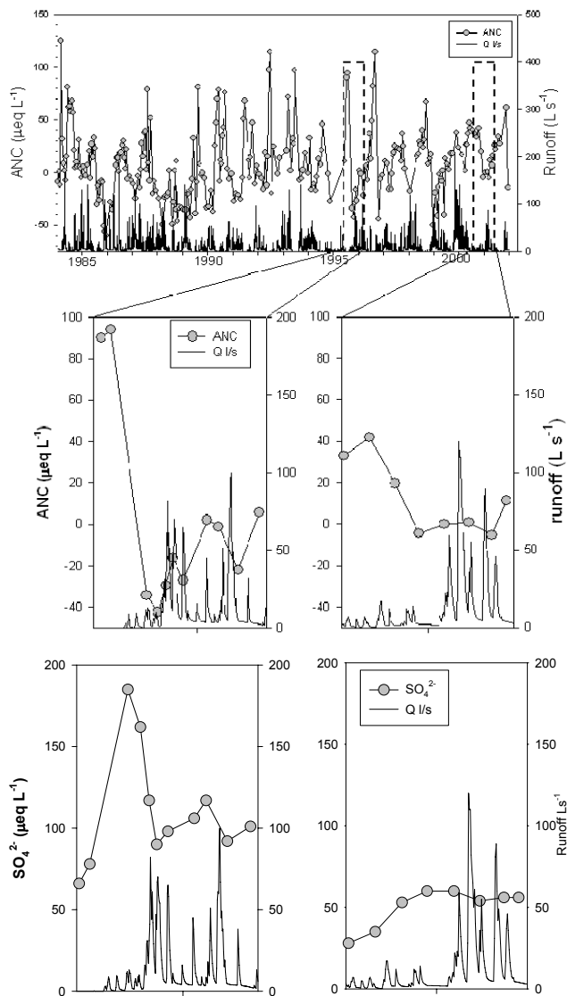
Fig. 3. (a) Time series of ANC variability from 1985–2002 in Tre-sticklan (above) with examples of episodic ANC response with dry antecedent conditions (below left) and wet antecedent conditions (below right). (b) The accompanied SO 4 response to the dry antecedent conditions (left) and wet antecedent conditions (right).
