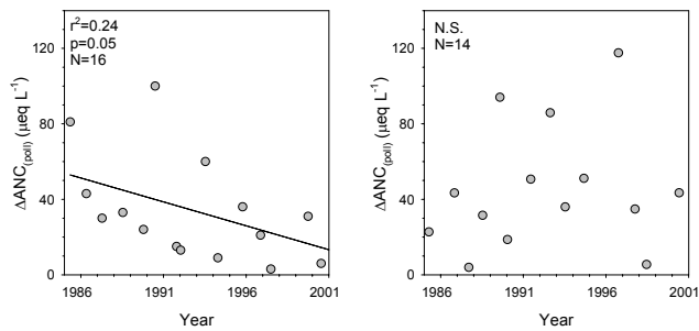
Fig. 2. Trend in anthropogenic response \Delta\text{ANC}_{(\text{poll})} during episodes in one inland stream (Bråtång) with declining \Delta\text{ANC}_{(\text{poll})} (left) and one coastal stream (Tostarp) with no trend in \text{ANC}_{(\text{poll})} over time (right).
