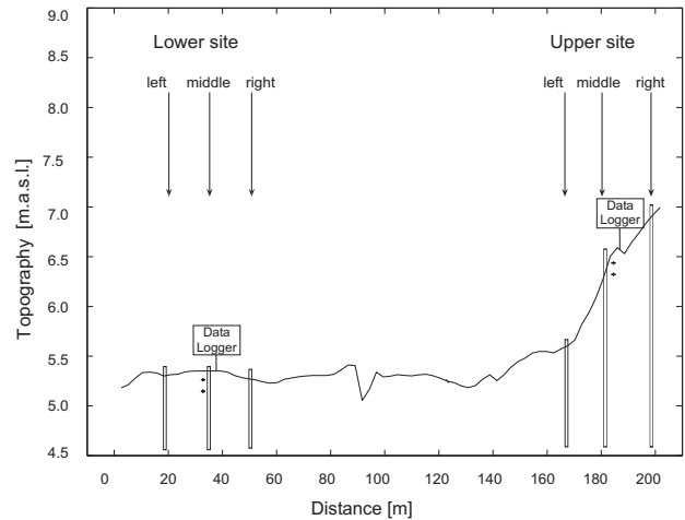
Fig. 1. Lower and the upper site along the topographical transect in the Bourgoyen-Ossemeersen. The left, middle and right sampling points at each site are indicated by arrows, long tubes are the piezometers and + indicates the soil water content reflectometers.
