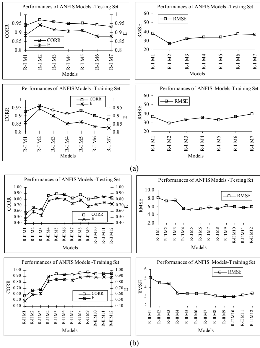
Fig. 7. Performances of ANFIS models, (a) Seyhan River, (b) Cine River.
