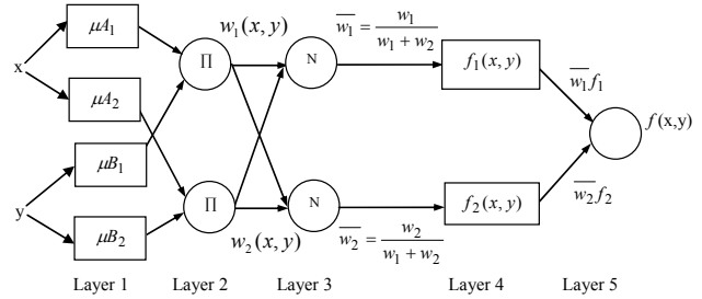
Fig. 2. The scheme of Adaptive Neuro-Fuzzy Inference System.
