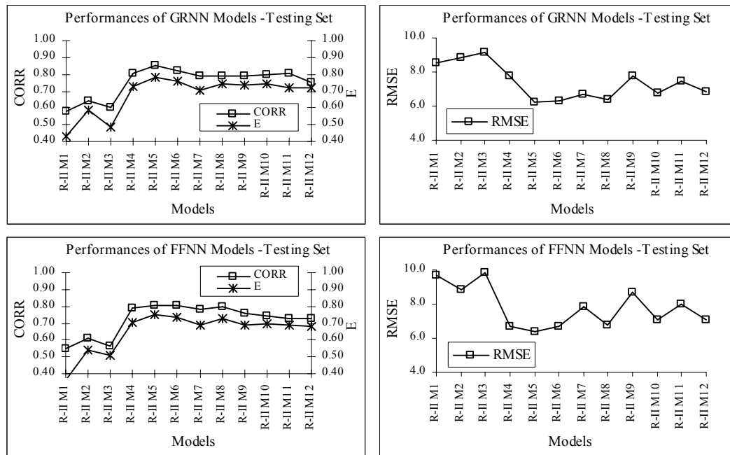
Fig. 9. The Performances of GRNN and FFNN models for Cine River.
