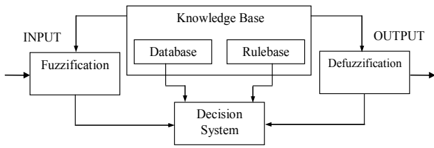
Fig. 1. The general structure of the Fuzzy Inference System.
