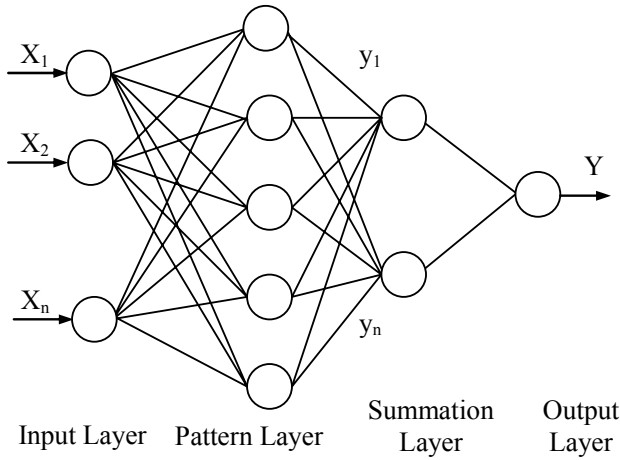
Fig. 4. The general structure of a GRNN.
