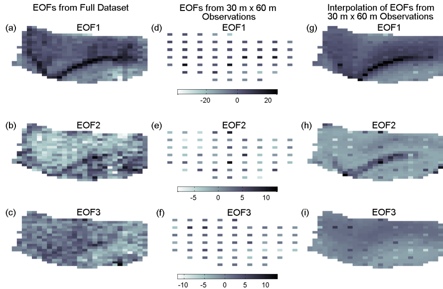
Fig. 4. (a–c) EOFs 1–3 computed from the full 10 m × 20 m soil moisture dataset, (d–f) EOFs 1–3 computed from an observation set with a 30 m × 60 m spacing, and (g–i) Interpolations of EOFs 1–3 from the 30 m × 60 m spacing back to the 10 m × 20 m spacing using a MLR against topographic attributes.
