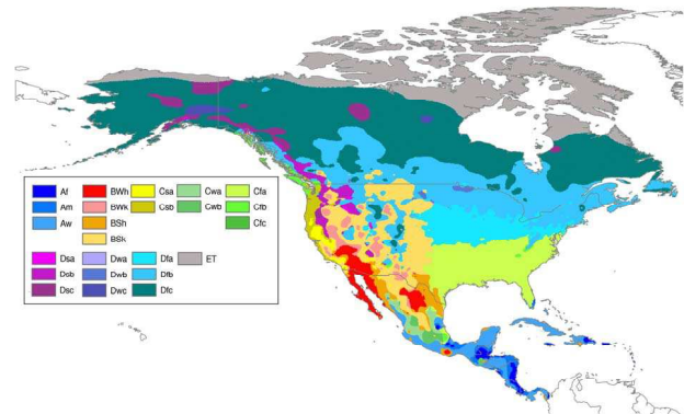
Fig. 6. Köppen-Geiger climate type map of North America.
