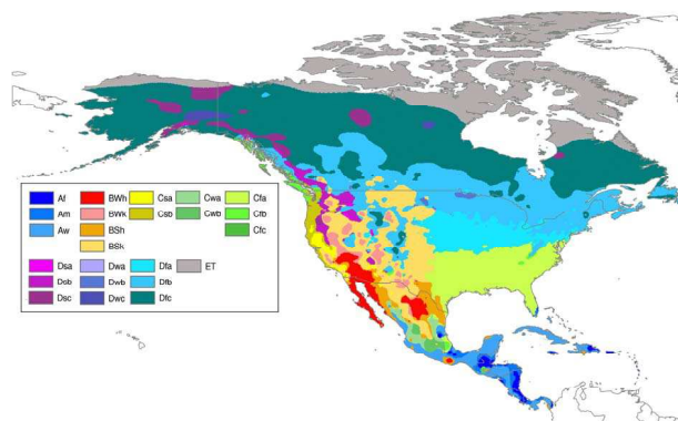
Fig. 6. Köppen-Geiger climate type map of North America.
