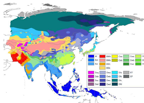
Fig. 5. Köppen-Geiger climate type map of Asia.
