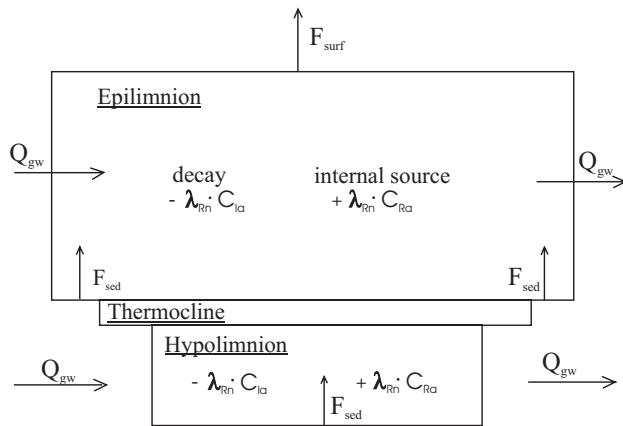
Fig. 6. Box model of the stratified lake. Radon sources are groundwater inflow Q_{\text{gw}} , sediment flux F_{\text{sed}} and the decay of dissolved radium in the lake water ( \lambda_{\text{Rn}} \times C_{\text{Ra}} ). The radon concentration is decreased by decay ( \lambda_{\text{Rn}} \times C_{\text{la}} ), outgassing to the atmosphere F_{\text{surf}} and the outflow. The radon exchange between the two boxes is neglected, because of the stratification and the reduced transport through the thermocline.
