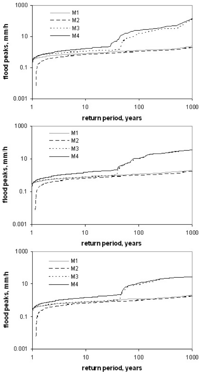
Fig. 7. Flood frequency curves for the four models using (a) \eta=0.5 , (b) \eta=1.5 , and (c) \eta=3 , and S_b=150 mm.
