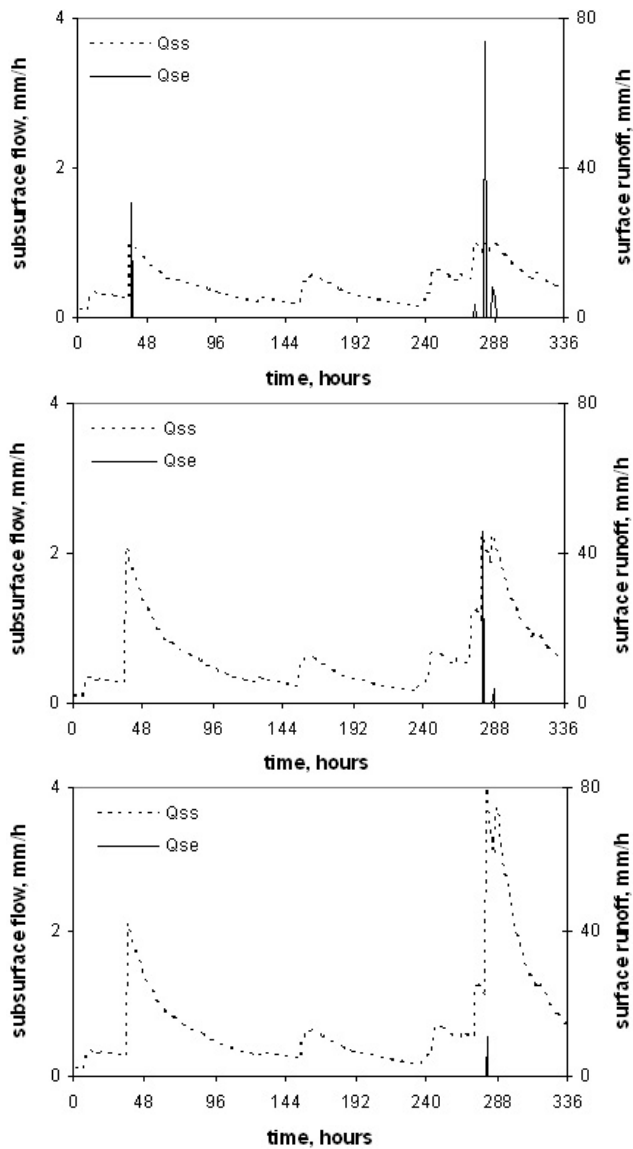
Fig. 5. The impact of bucket capacity generated by Model 4 using \eta=0.5 and (a) S_b=100 m, (b) S_b=150 mm, and (c) S_b=200 mm.
