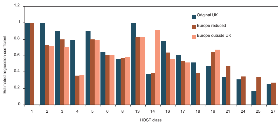
Fig. 5. Comparison of estimated regression coefficients per HOST class from the original UK study and from European catchments inside and outside the UK based on the reclassified SGDBE. Original UK designates the coefficients obtained by Boorman et al. (1995: Table 3.8). Europe reduced are the estimates for the reduced set of catchments from the UK and Europe (Groups C + D; rhomboids and circles in Figs. 3 and 4), constraint to lay between 0 and 1 and optimised using step-wise Akaike. Europe outside UK designates the values estimated from catchments outside the UK only (Group D; circles in Figs. 3 and 4), using constraints 0 and 1 and step-wise optimisation. Only those classes are shown for which coefficients from the Europe reduced dataset could be obtained.
