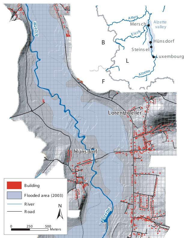
Fig. 2. The study area. The Alzette River and adjacent buildings superimposed upon a 50 m resolution DEM of the floodplain.
