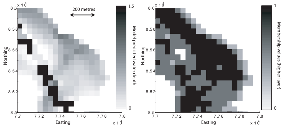
Fig. 4. A diagram illustrating the transformation from model results for a single LISFLOOD-FP realisation (a) to the fuzzy interpretation map of inundation categories (b) arising from the use of the subjective function illustrated in Fig. 3. Only the high inundation possibility layer is illustrated. The cell size is 50 m.
