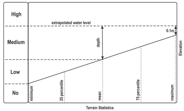
Fig. 3. A function relating model predicted water depths to fuzzy, inundation possibility, category vectors. The LISFLOOD predicted depth value from a cell or, if dry, from adjoining cells is used to calculate the water level across a cell and the intercept of this water level on the terrain statistics surface is used to allocate fuzzy category vectors. The pixel resolution is 50 m.
