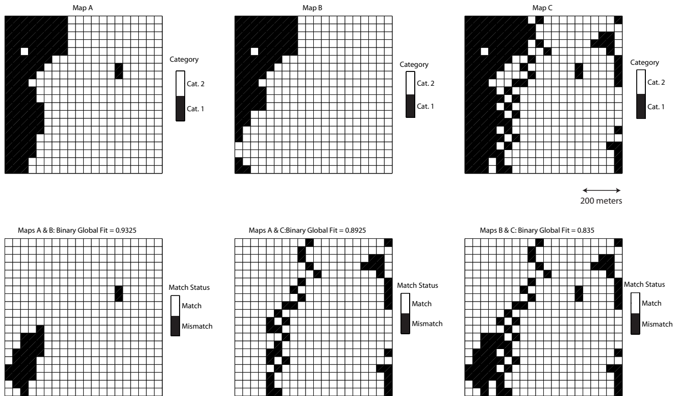
Fig. 1. An example of map comparison using a discrete, binary matching system. Maps A, B and C can be regarded as interpretations of the same data set in which there is uncertainty in the category status across zones delineated. The lower maps show how the global fit (assessed as the ratio of matching cells to the total number of cells) cannot represent the uncertainty in cell status. The match between A and B may be an overestimate due to coincidental matching of categories within the zones of uncertainty while the match between B and C may be an underestimate due to poor matching of cells within the uncertainty zones.
