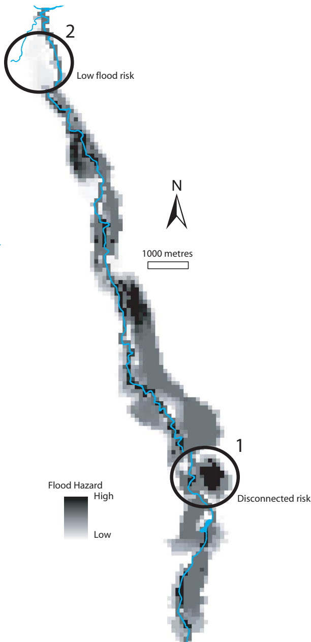
Fig. 7. An inundation likelihood map for Alzette created from conditioning LISFLOOD-FP on a fuzzy representation of the SAR data using the fuzzy performance measure.
