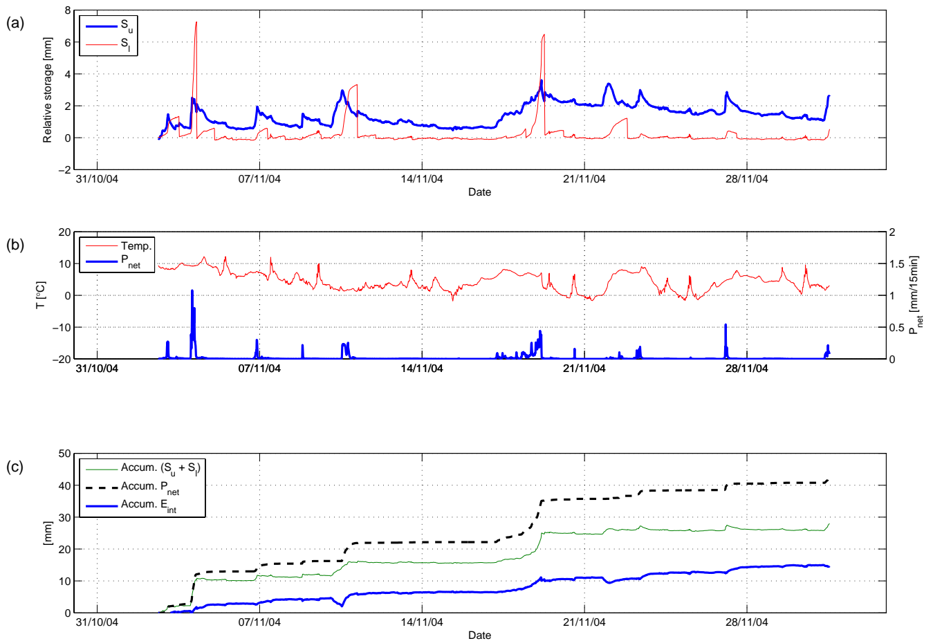
Fig. 5. Measuring results of the Huewelerbach catchment for November 2004. (a) Storage in the upper and lower basin compared to initial situation (relative storage); (b) Meteorological data (net rainfall and temperature); (c) Cumulated evaporation from interception compared to total net rainfall.
