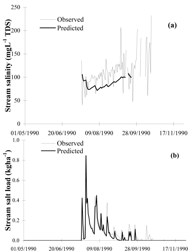
Fig. 8. Actual and predicted stream (a) salinity and (b) salt load for 1990 – Ernies catchment.
