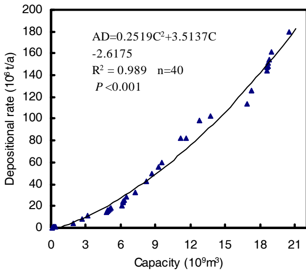
Fig. 5. Correlation between deposition rate and storage capacity of the reservoirs in the upper Yangtze.
