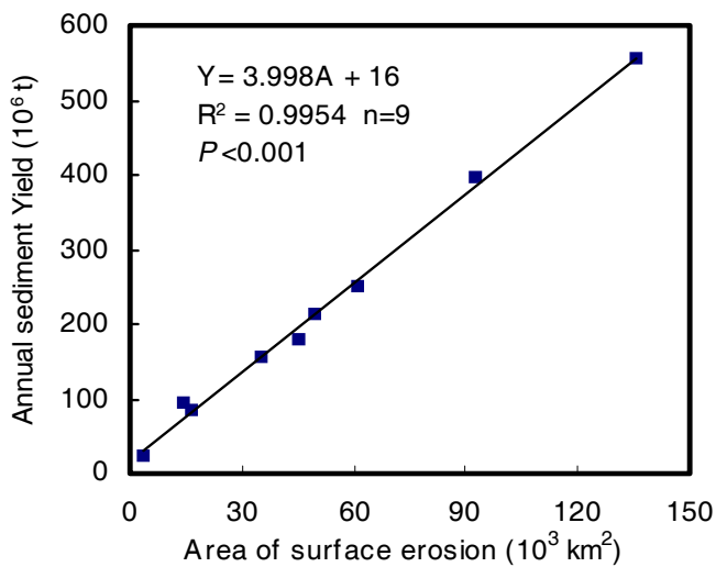
Fig. 3. Regression between area of surface erosion ( A ) and annual sediment yield ( Y ) (data in Table 2).
