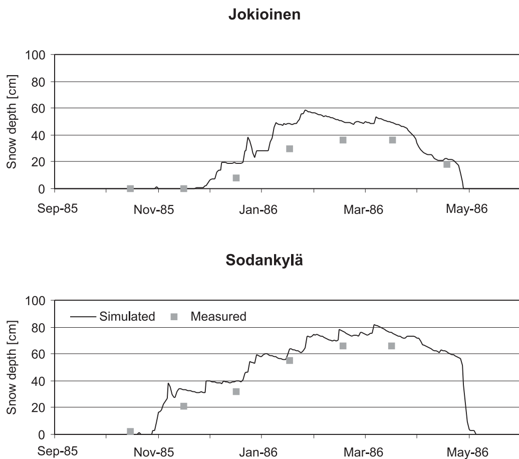
Fig. 6. Simulated and observed snow depths at Sodankylä and Jokioinen
