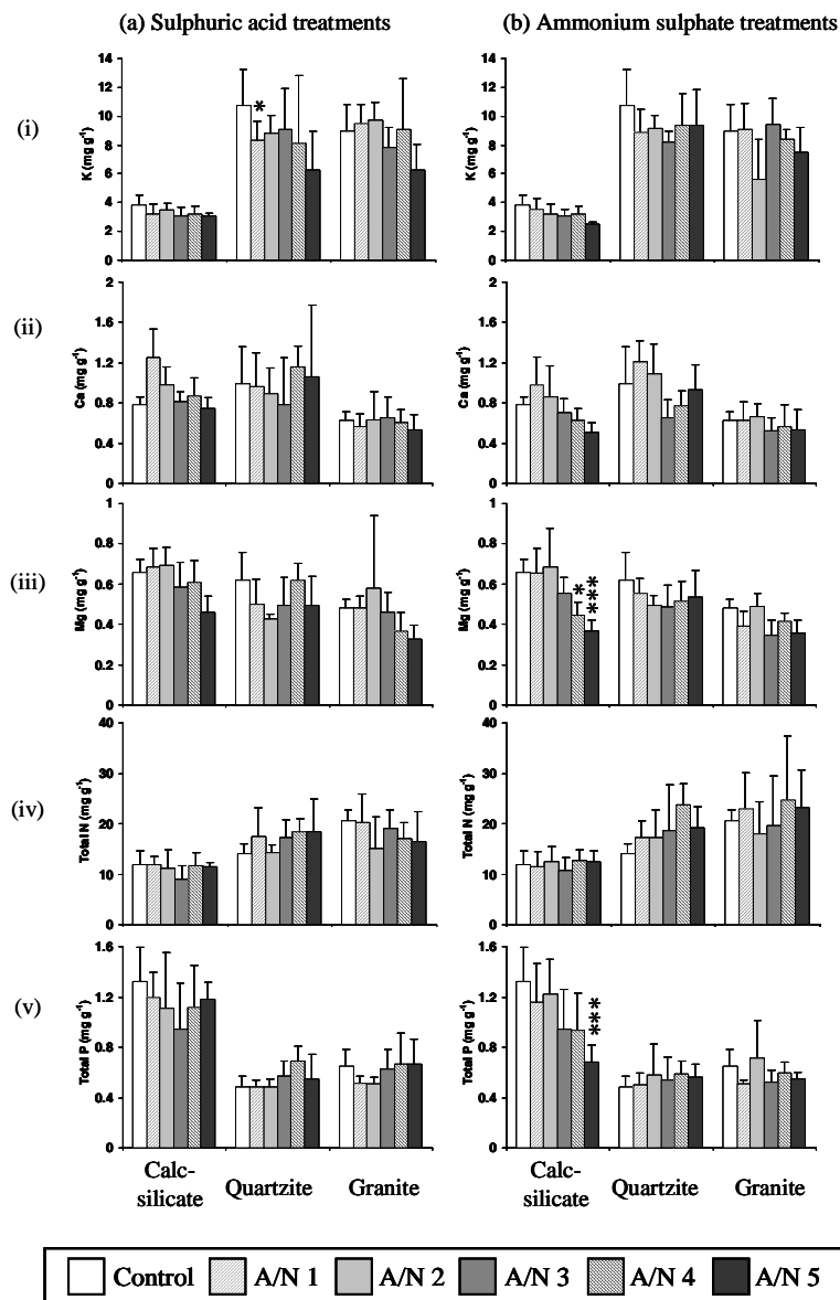
Fig. 8. The effects of (a) sulphuric acid and (b) ammonium sulphate treatment levels on seedling mean foliar content ( \pm 1s error bars) of (i) K, (ii) Ca, (iii) Mg, (iv) total N and (v) total P ( mg\ g^{-1} of dry mass material). Significant differences between seedlings in treated microcosms compared to control microcosms are given as * p \leq 0.05 , *** p \leq 0.001 and no symbol denotes not significant.
