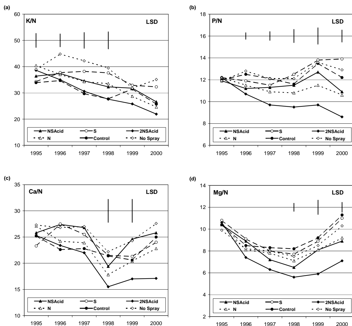
Fig. 5. Nutrient ratios for K, P, Ca and Mg in relation to N (*100) for current year foliage in Sitka spruce treated with N S / Acidity for years 1995 (pre-treatment) to year 2000. LSDs are given where treatment effects were significant P < 0.05 .
