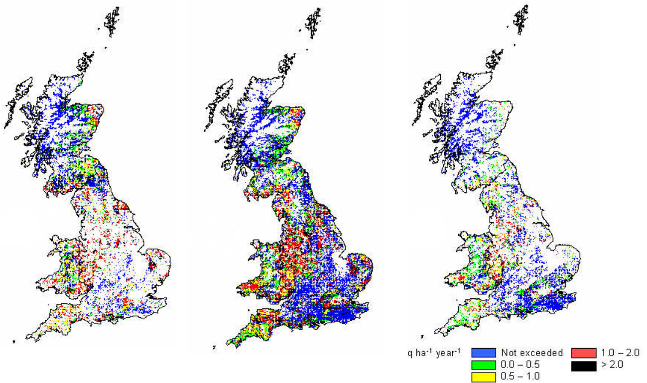
Fig. 5. Critical load exceedance using modelled total acid deposition data for 2010, for: (a) managed coniferous woodland, (b) managed broadleaved and mixed woodland and (c) unmanaged woodland.
