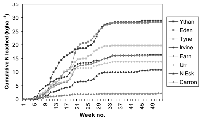
Fig. 7. Predicted cumulative N leached for 8 catchments from autumn 1990 to autumn 1991
