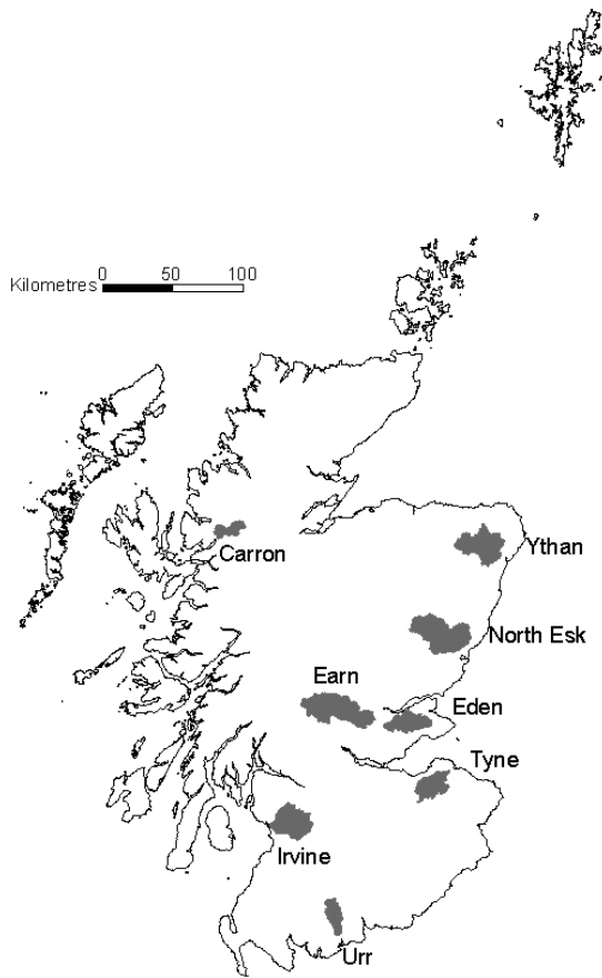
Fig. 6. Locations of NIRAMS test catchments
