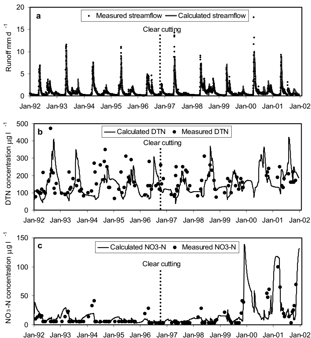
Fig. 4. Stream runoff ( \text{mm d}^{-1} ) (a), measured and simulated concentrations of dissolved total nitrogen (DTN) (b) and nitrate-N ( \text{NO}_3\text{-N} ) (c) in Kangasvaara outlet stream ( \mu\text{g N l}^{-1} ). Clear-cutting in the catchment was performed during August–October 1996.
