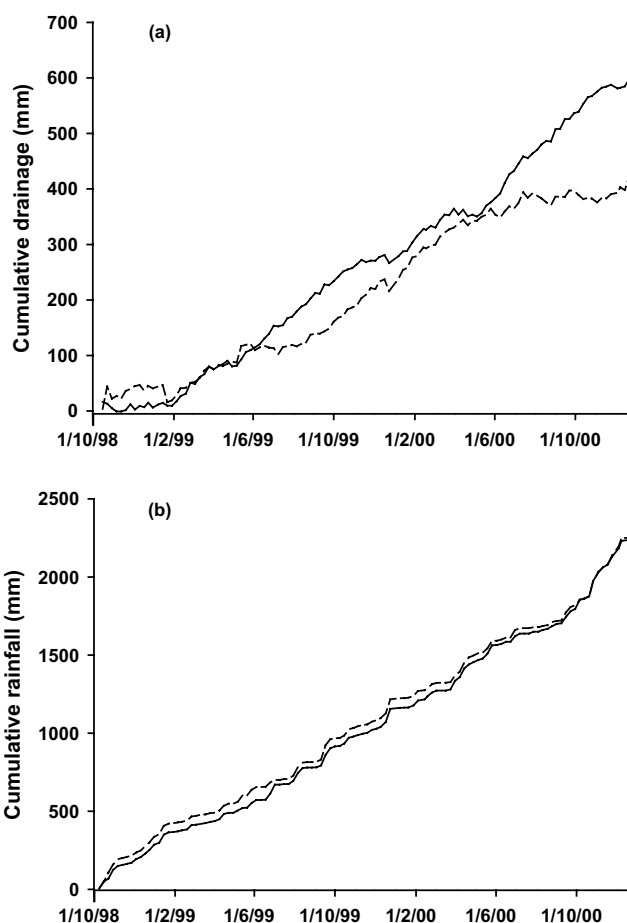
Fig. 5. (a) Cumulative drainage calculated from a water balance below woodland at Black Wood (—) and pasture at Bridgetts Farm (---) from October 1998 up to December 2000. (b) Cumulative rainfall at Black Wood (—) and Bridgetts Farm (---) over the same period.
