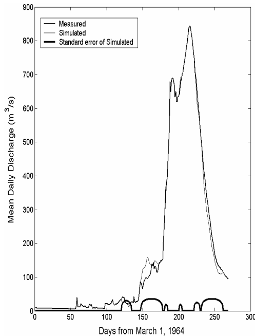
Fig. 3j. Measured and Simulated Daily Hydrographs for Lawra on the Black Volta River (Black Volta Basin) - State Space Model on Lawra and Bamboi Daily Discharges (Missing Data Pattern 2).
