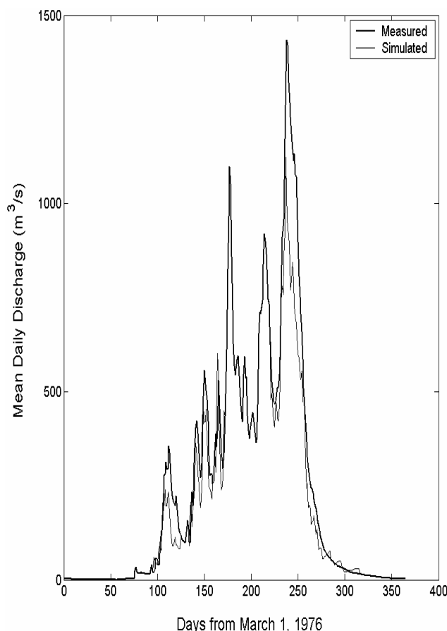
Fig. 5d. Measured and Simulated Daily Hydrographs for Sabari on the Oti River (Oti Basin) – Linear Regression on 1976 Saboba and Non-missing Sabari Daily Discharges.
