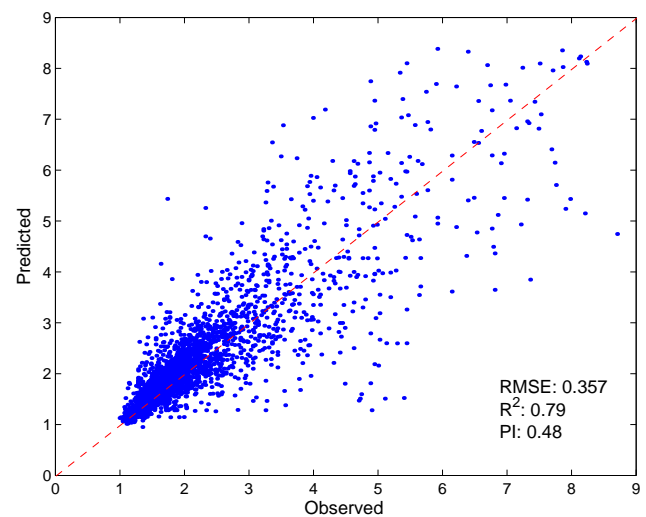
Fig. 12. Scatter plot of predicted versus observed hourly discharges ( \text{m}^3/\text{s} ) for a six-hour-ahead forecast based on historical rainfall and discharge values.
