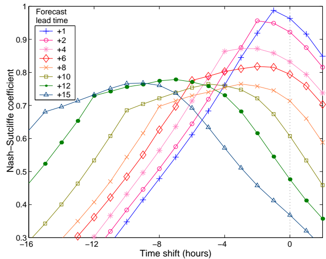
Fig. 15. ANN multi-step-ahead forecast performances (in terms of the Nash-Sutcliffe coefficient) for various shifts in time of the forecasted versus the observed time series.
