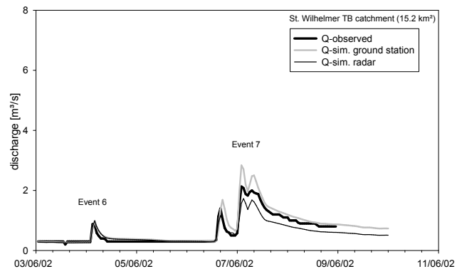
Fig. 6. Hydrographs of the events 6 and 7 for the St. Wilhelmer Talbach catchment ( 15.2 \text{ km}^2 ).
