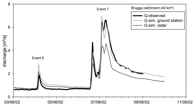
Fig. 5. Hydrographs of the events 6 and 7 for the Brugga catchment ( 40 \text{ km}^2 ).
