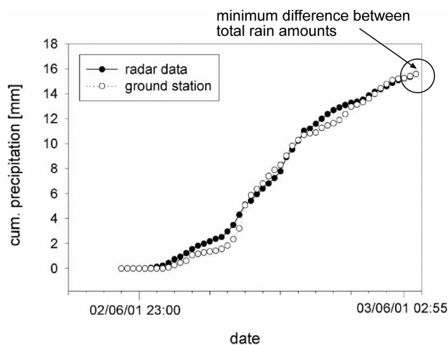
Fig. 3. Radar data calibration using the minimum square distance method for the cumulative curves of both rainfall data sets, showing minimized difference between the total precipitation amounts of both data sets as an additional constraint.
