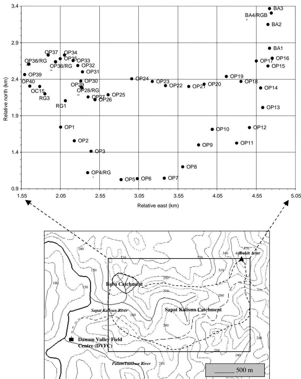
Fig. 1. Distribution of the storage raingauges (OP, BA, OC) and the recording raingauges (RG) monitoring rainfall within the 4-km 2 Sapat Kalisun Experimental Catchment. The gauge number begins with a symbol, where OP is a haulage road site, BA is an canopy opening on Atur Hill (Bukit Atur) and OC is canopy gap away from haulage roads.
