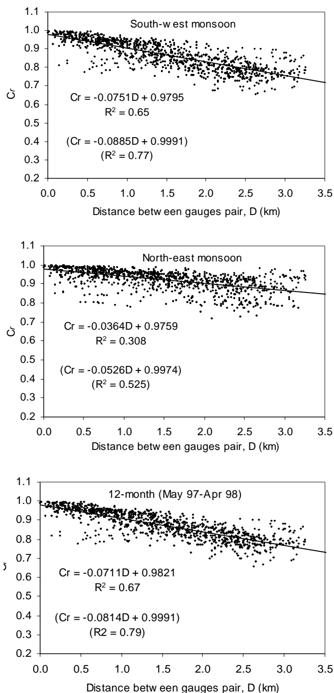
Fig. 4. Correlation ( C_r ) amongst point rainfalls as a function of distance between gauges ( D ) for different periods of monitoring. Equations and r^2 of the relationships in brackets exclude the data from the Bukit Atur raingauges.
