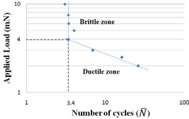
Figure 6: Wöhler diagram of the contact fatigue results
