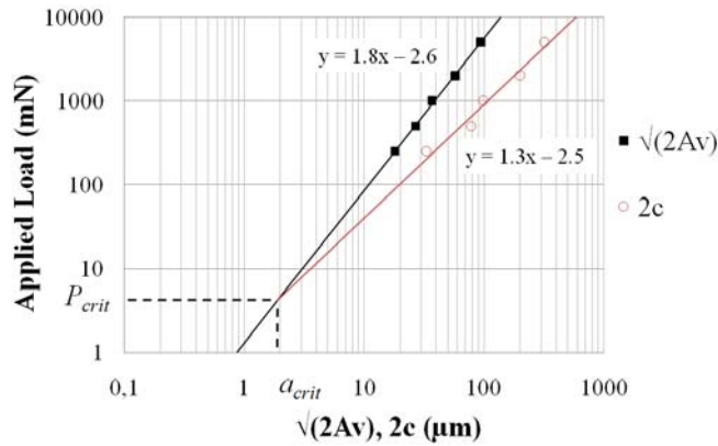
Figure 4: Vickers indentation results: plasticity length \sqrt{2A_v} (solid squares), fracture 2c (open circles). Extrapolations of these results give the critical size of \text{CaCO}_3
