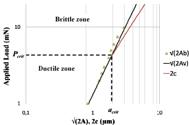
Figure 5: Comparison between plastic deformation sizes induced by nanoindentation and Vickers indentation on \text{CaCO}_3 for single-cycle study
