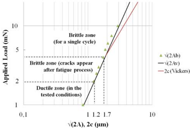
Figure 7: Evolution of the brittle-ductile transition with fatigue
