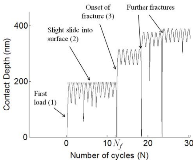
Figure 3: Contact depth as a function of the number of cycles ( N ) for a maximum load = 2.5 mN (here cracking occurs for N_f=12 ). Further fractures are often observed after the first one occurred.
