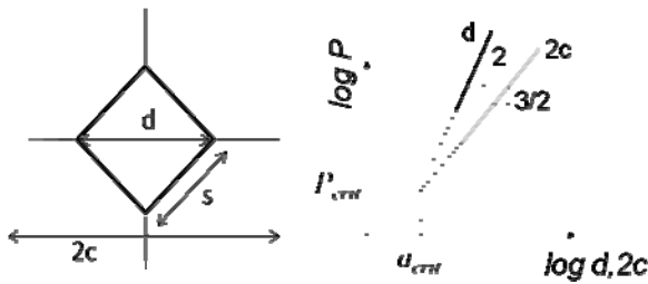
Figure 1: a) Scheme of a Vickers indent with radial cracks; b) Theoretical evolution of diagonal length d of the Vickers indentation and crack length 2c versus the applied load P
