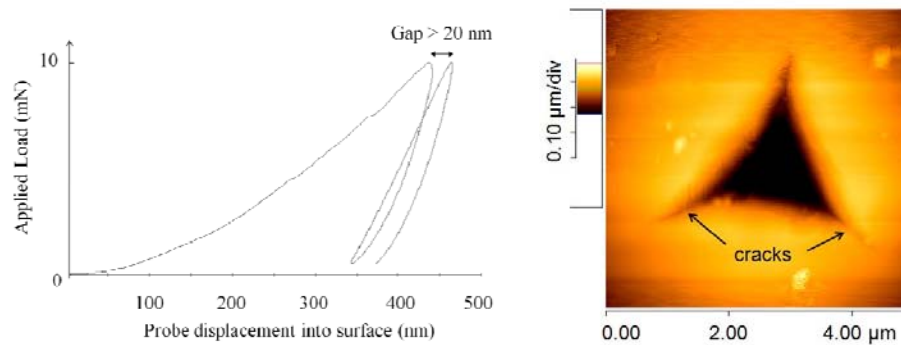
Figure 2: a) Indentation curve on CaCO 3 , b) Corresponding AFM image of the Berkovich indent with cracks (maximum load = 10 mN)
