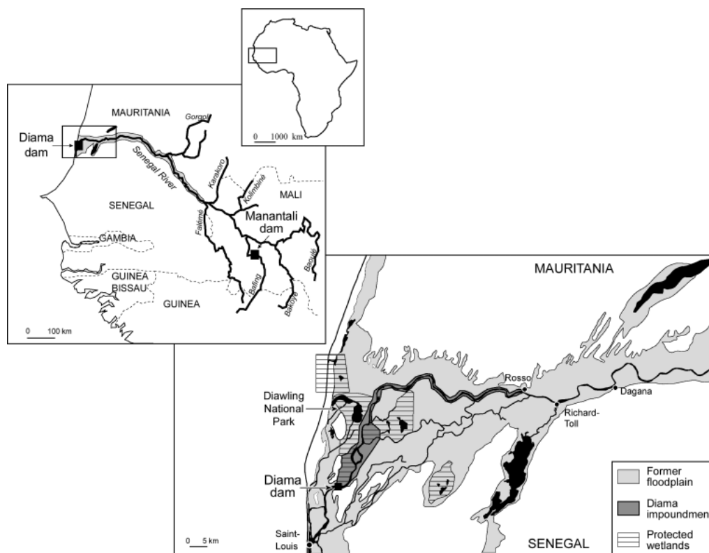
Fig. 1. Map of Africa, with as inset a map showing the Senegal River Basin with the location of the two large dams. The second inset map shows the Senegal River Delta with the former floodplain, the Diama dam impoundment and the various protected wetlands, including the Diawling National Park.
