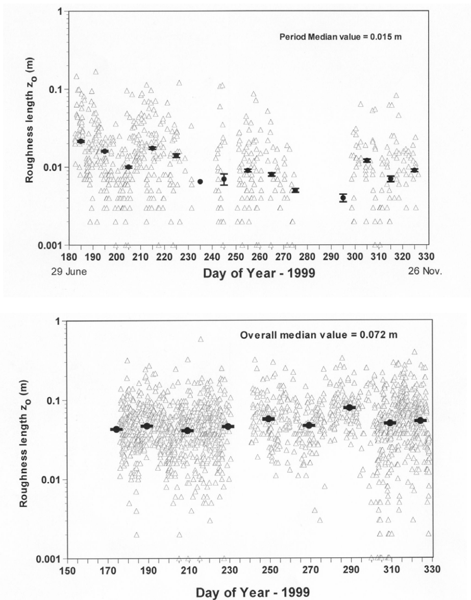
Fig. 5. Calculated roughness lengths: Tadham Moor (top), Ham Wall (bottom).
