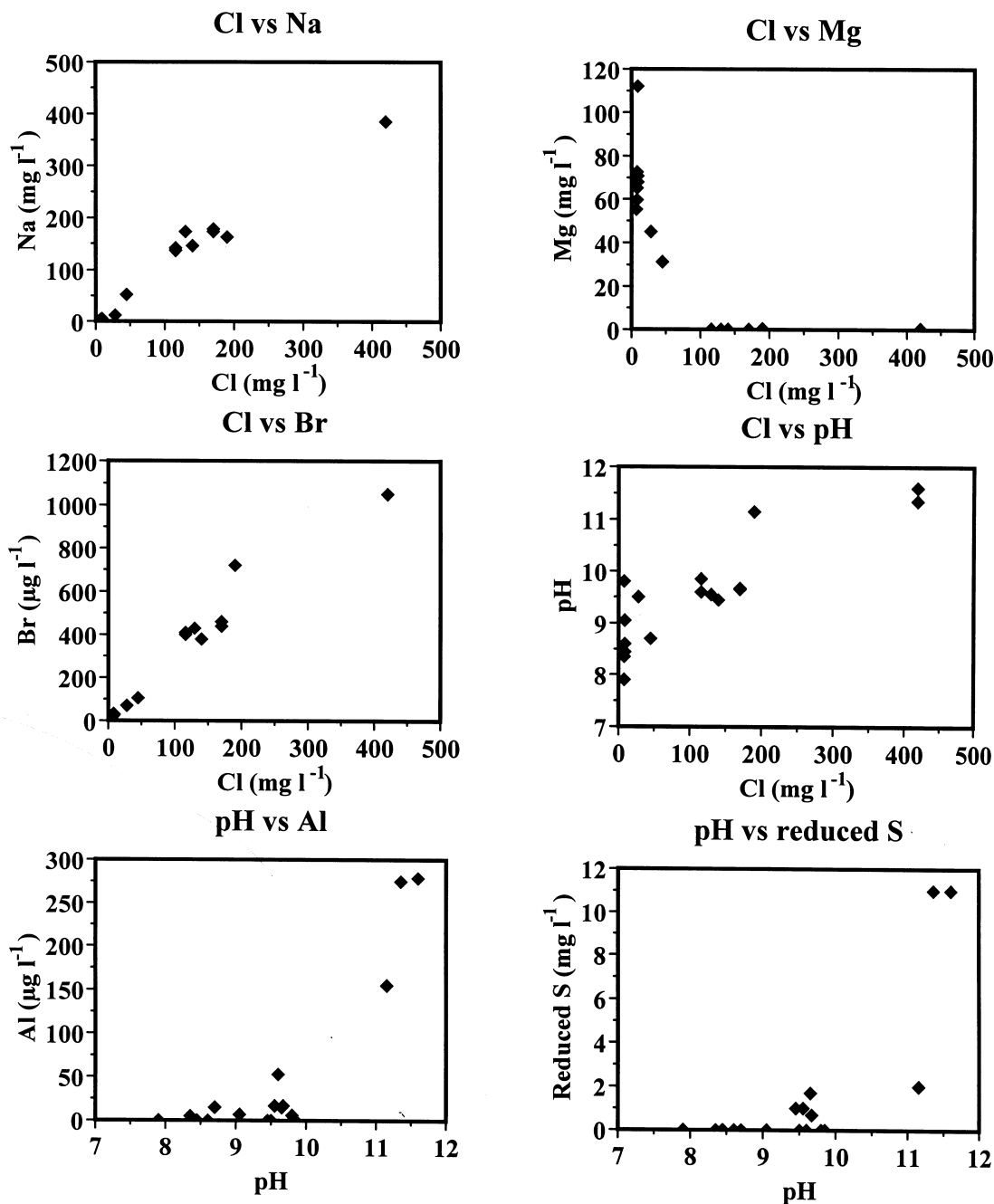
Fig. 3. Inter-determinand plots for Type 1, 2 and 3 water groupings
