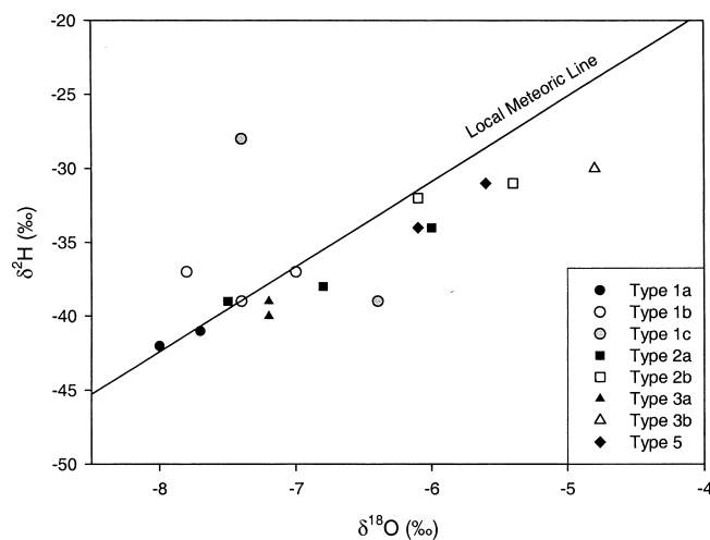
Fig. 5. Relationship between \delta^2H and \delta^{18}O for the Troodos groundwaters. Local meteoric water line from Jacovides (1979). The sample of Type 4 water is not plotted because of a potential spurious analysis for \delta^2H .
