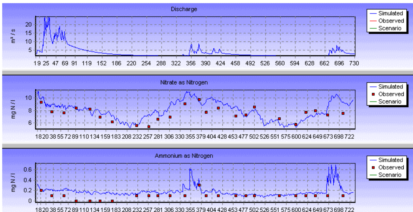
Fig. 5. Reach 7: simulated and observed data (1995–96)
