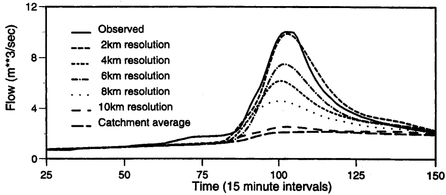
Fig. 9. Hydrographs obtained using different resolutions of raingauge data, 20–29 May 1994.
