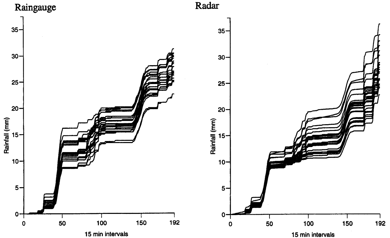
Fig. 3. Cumulative raingauge and radar hyetographs for grid squares containing raingauges in the Brue catchment for periods of convective and stratiform rain.
