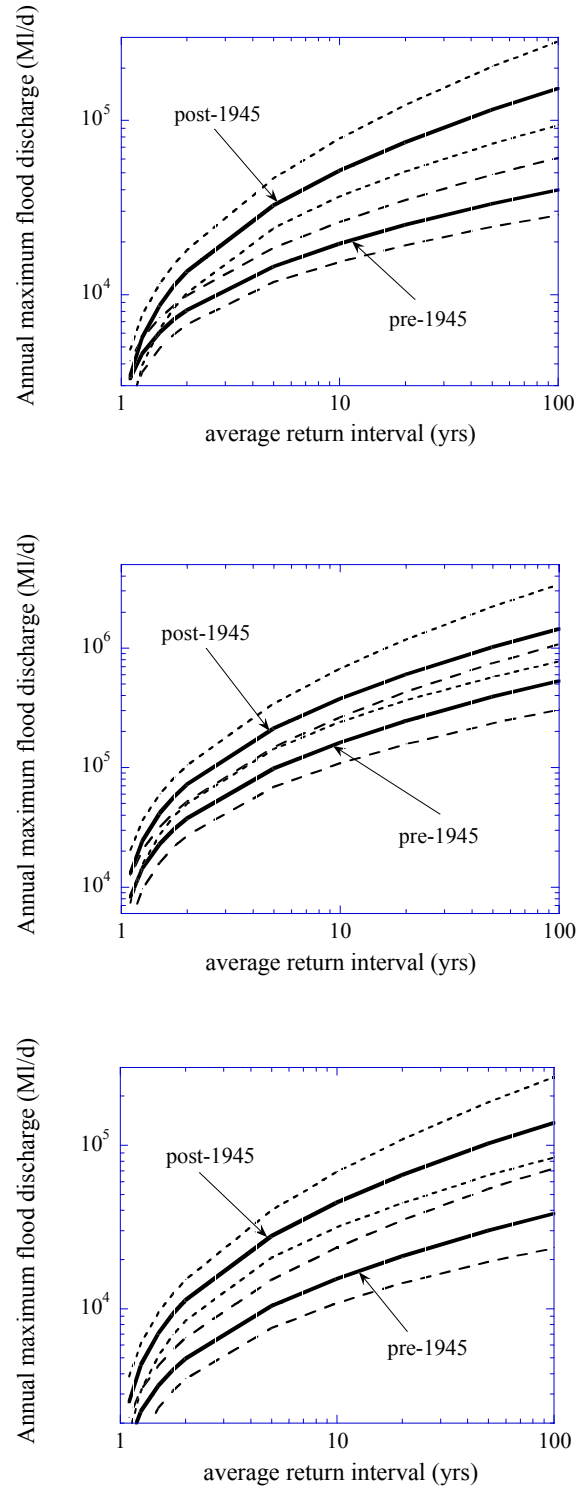
Fig. 3. Log-normal expected quantiles and their 90% probability limits (dashed lines) for three sites in study region, stratified at 1945.
