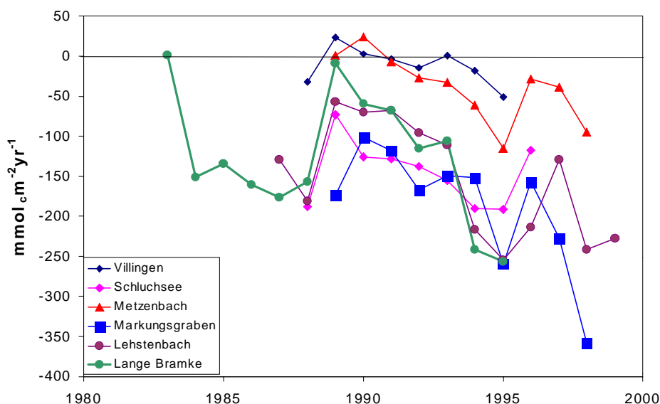
Fig. 6. Element budgets for sum of base cations ( \Sigma Ca, Mg, Na, K) in \text{mmol m}^{-2} \text{yr}^{-1} calculated as total deposition minus run-off flux.
