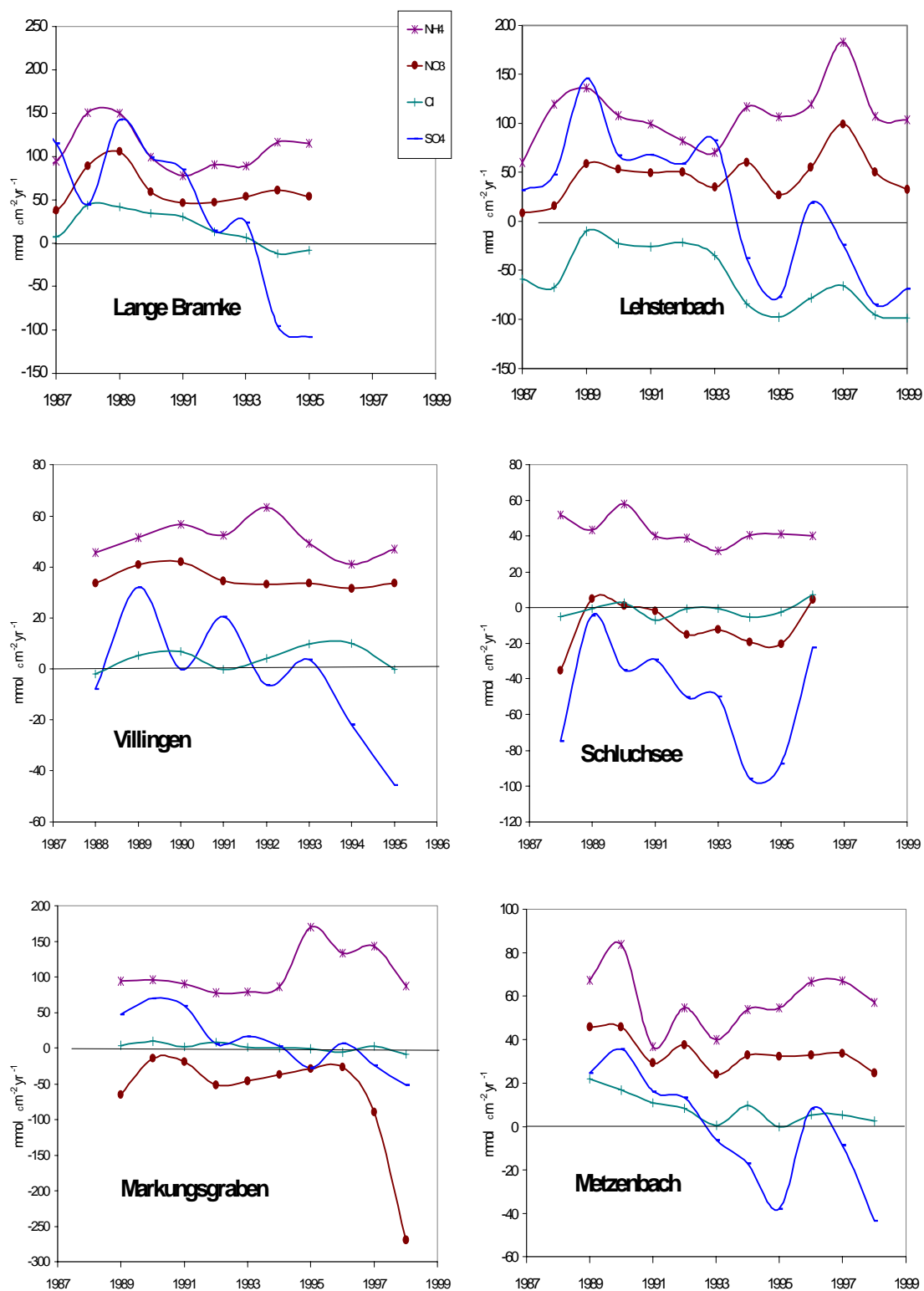
Fig. 5. Element budgets (mmol cm -2 yr -1 ) for NH 4 , NO 3 , Cl and SO 4 calculated as total deposition minus run-off flux
