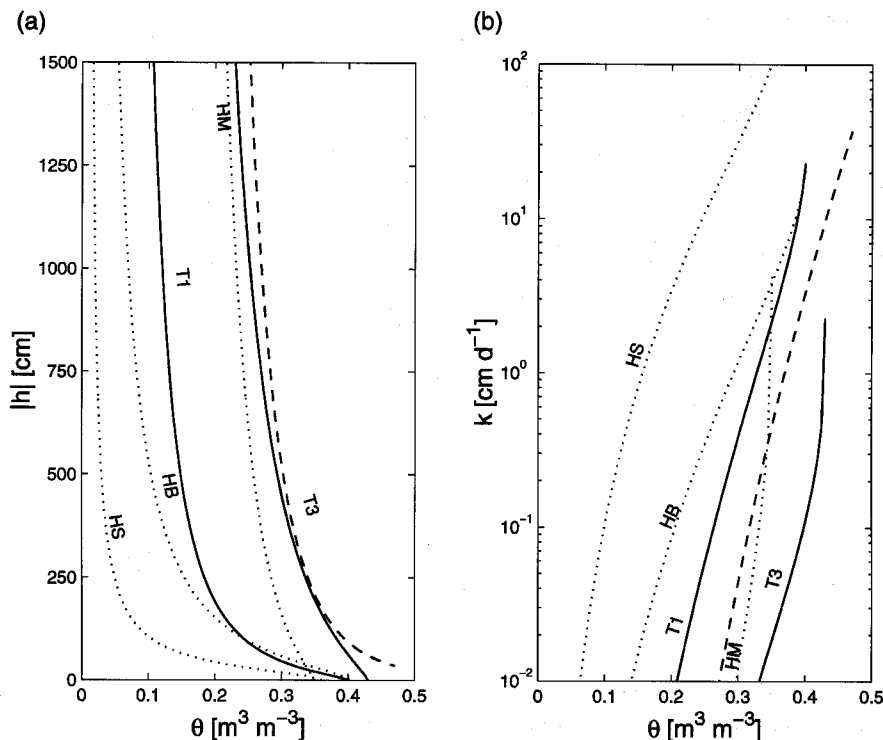
Fig. 7. (a) Soil water pressure head and (b) hydraulic conductivity as functions of soil moisture \theta using site specific MVG parameters (dotted), European soils data base HYPRES (solid) or standard RACMO curve (dashed). Sites are: HAPEX Mobilhy (HM), HAPEX Sahel (HS) and Hupselse Beek (HB); HYPRES texture classes are coarse (T1) and medium fine topsoil (T3).
