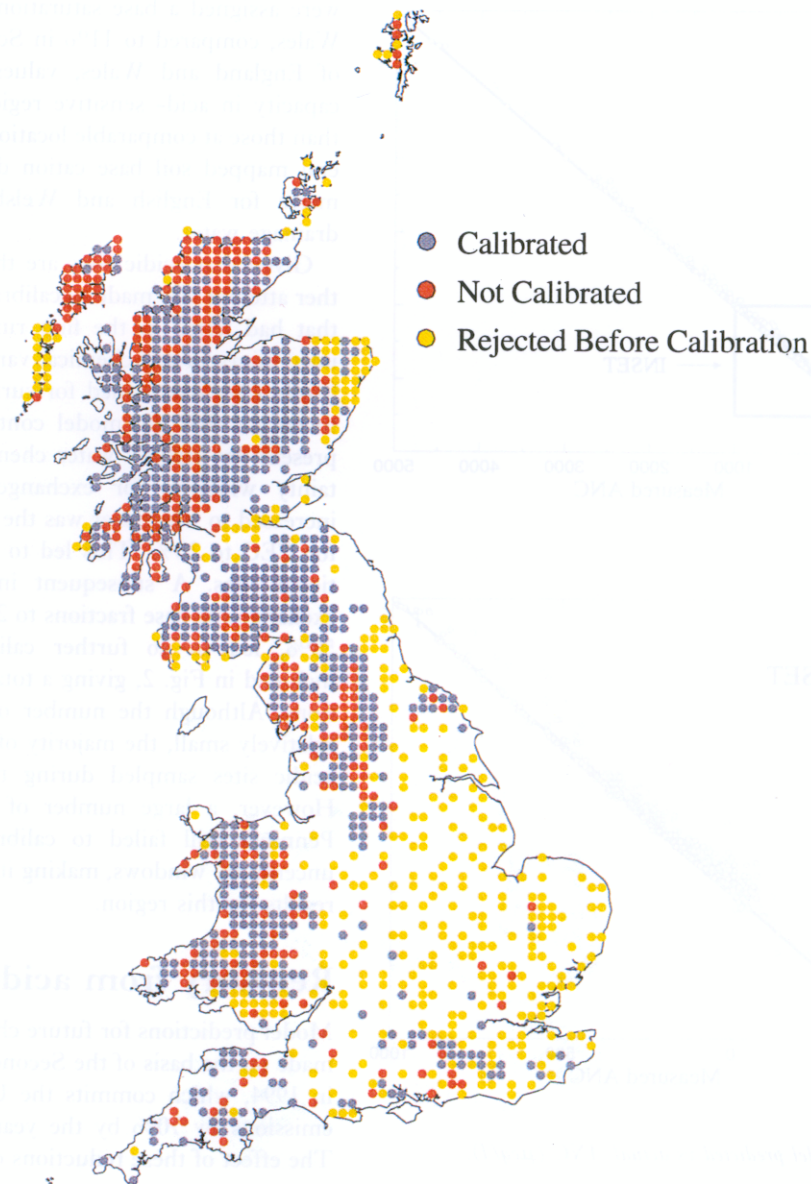
Fig. 2. Sites successfully calibrated by MAGIC.
