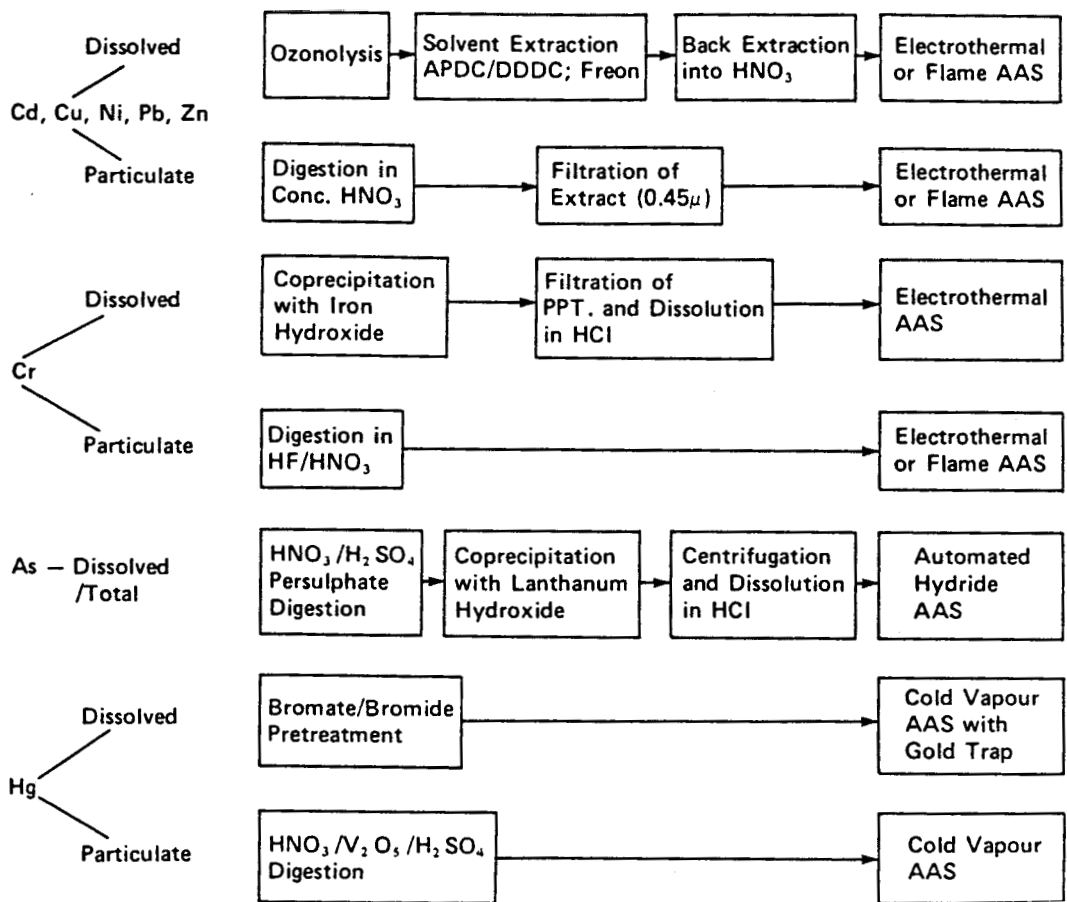
Fig. 4. Analytical methods
