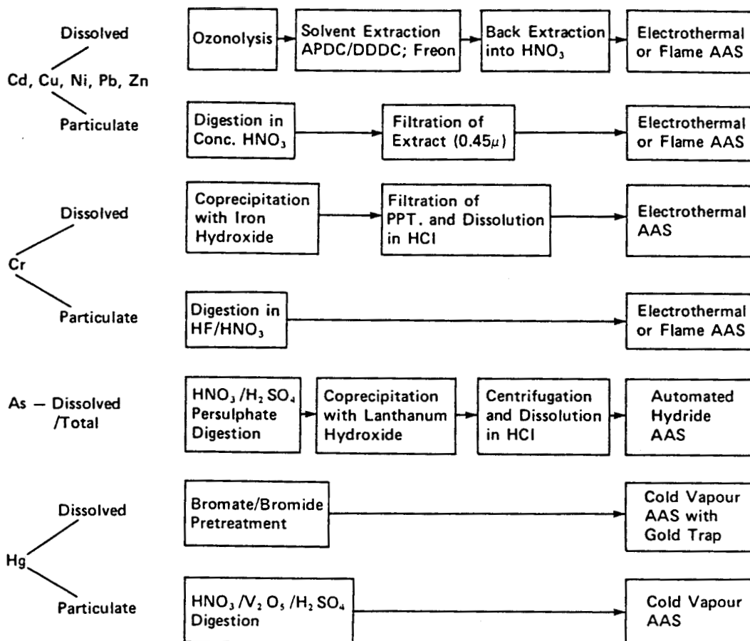
Fig. 4. Analytical methods
