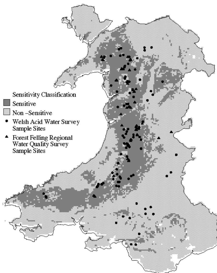
Fig. 2. Map of Wales showing the modified two band acid sensitivity classification and the location of sample sites for the Welsh Acid Waters Survey and the Forest Felling Regional Water Quality Survey.
